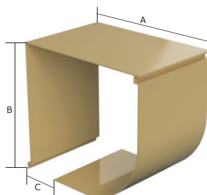
VR130 Model P Rounded box
