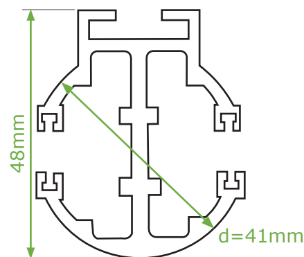
RE 41 Box support guide
