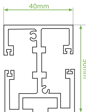
EF40 Box support guide
